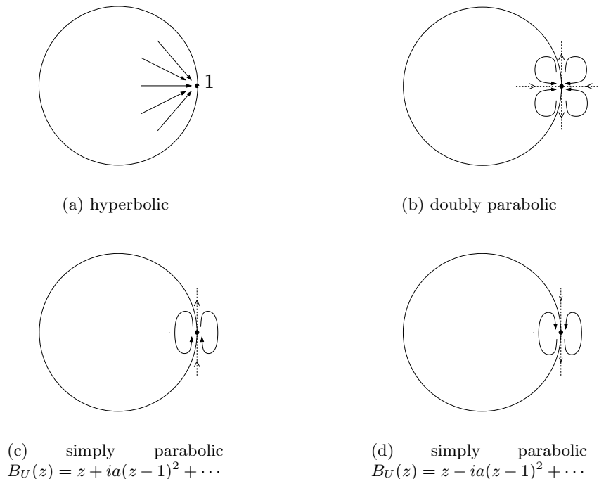
Figure 1: The three possibilities for the dynamics of B_U when U is a regular Baker domain. By the symmetry of the map, \mathbb{D} and \widehat{\mathbb{C}} \setminus \overline{\mathbb{D}} must belong to the basin of attraction of 1 and hence the Julia set must be a subset of the unit circle.
